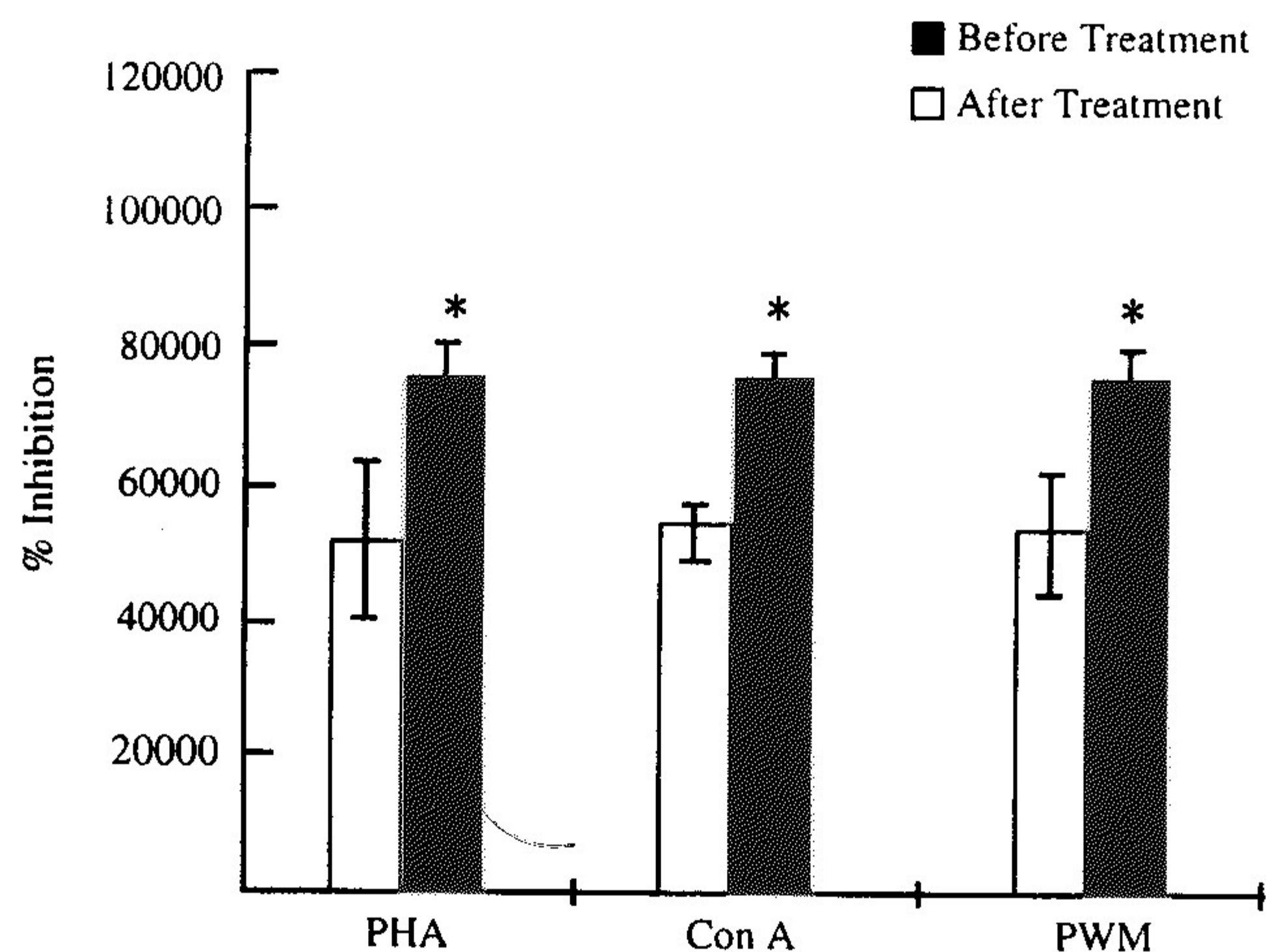
Fig. 4 In vivo action of MGN-3 on T and B cell mitogen response at one month after treatment.
